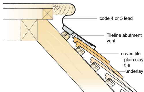
FLAT TO PITCHED ROOF JUNCTION
